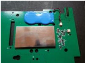
Modified version of the phone’s largest circuit board (with surveillance device). The battery pack (in blue) and the shielded module (in light brown) are part of the surveillance device.
