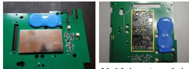
Modified version of the phone largest circuit board (with surveillance device). The battery pack (in blue) and the shielded module (in light brown) are part of the surveillance device.
