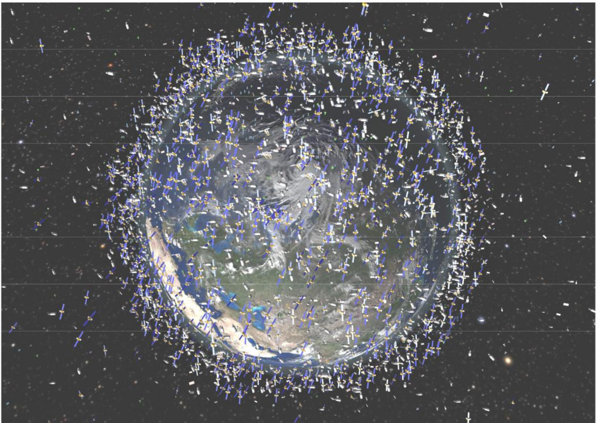
A COMPUTERISED MAP OF SOME OF THE SATELLITES IN ORBIT AROUND THE EARTH, AS OF 2009.
